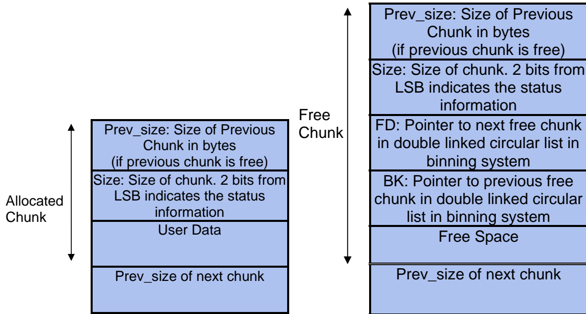
(a) Memory Layout for Allocated Chunk in Heap (b) Memory Layout for Free Chunk in Heap
