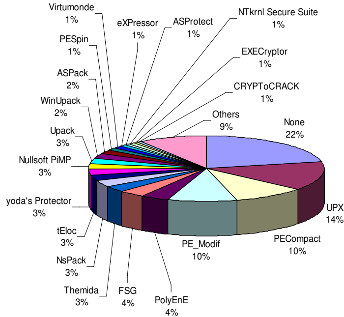
Figure 1.1 Statistic of techniques that malware used in year 2006
